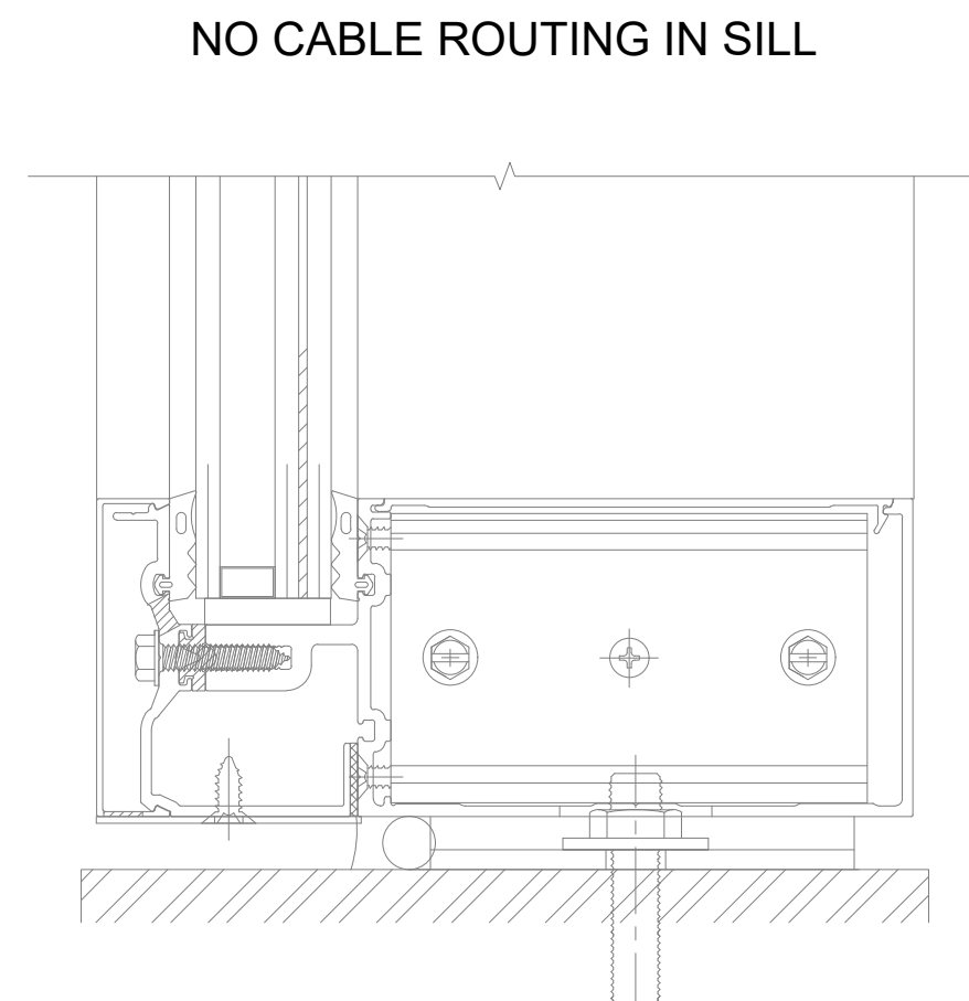
DETAIL 3 SILL
