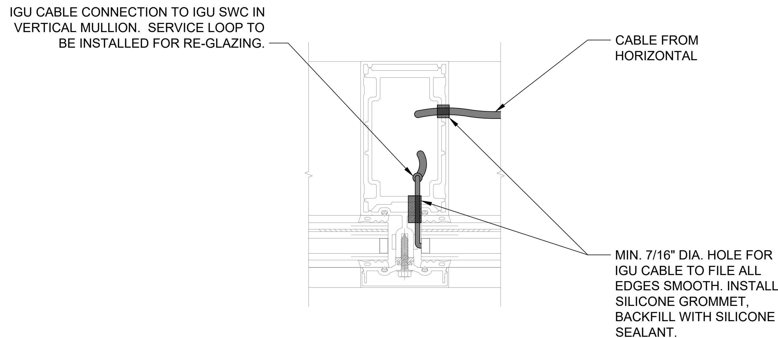
DETAIL 5 VERTICAL MULLION
